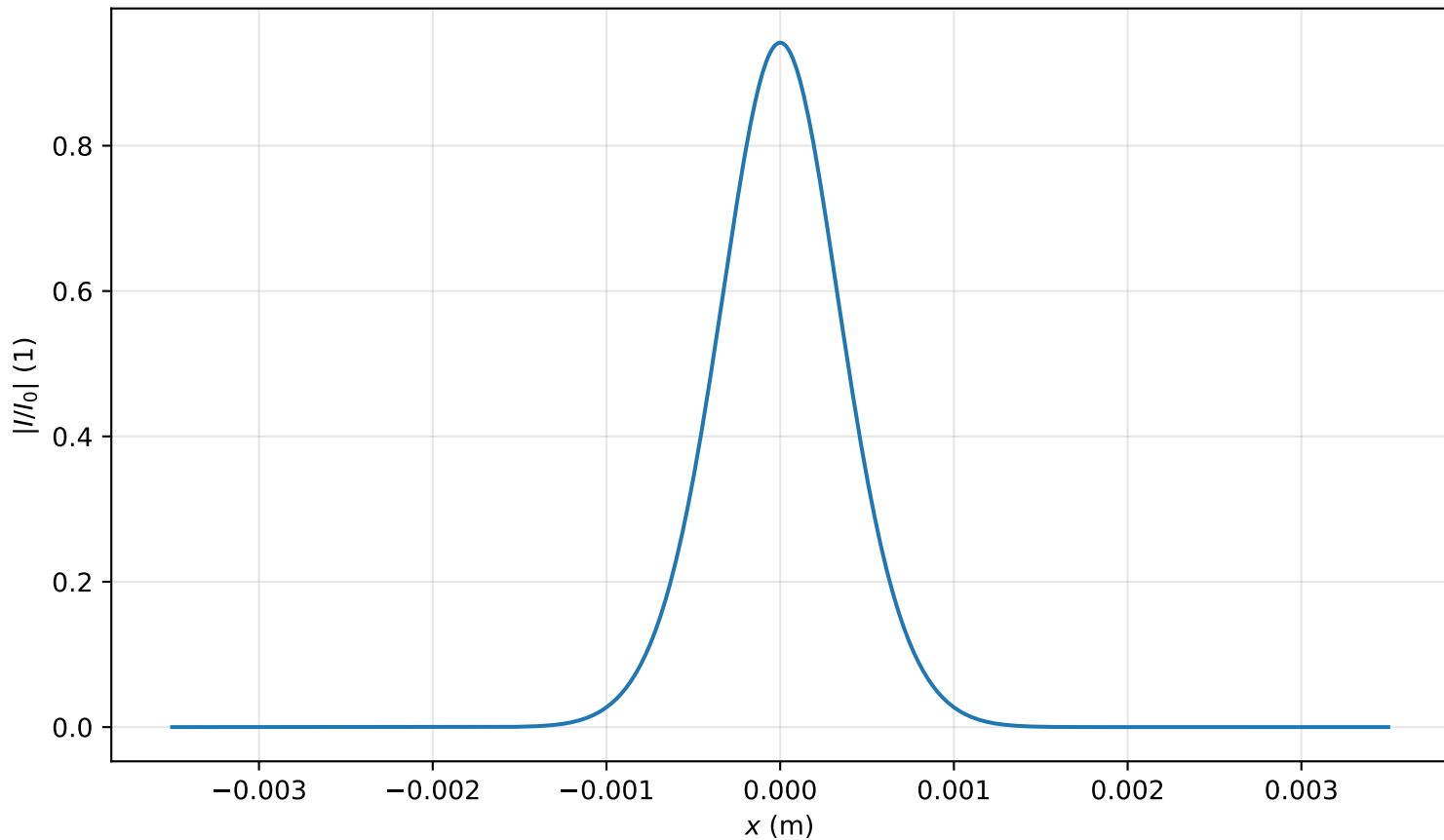
Intensity profile I(x, y = 0, z = 0.955m)/I_0 , P_{in}=0.3P_{cr} , artificial time
